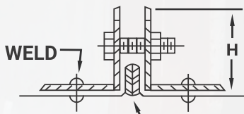
COMPANION ANGLES (CAULK OR GASKET) T-22
