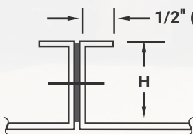
COMPANION ANGLES (CAULK OR GASKET) T-22
