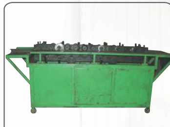
TDF Rollformer
