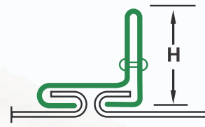
STANDING DRIVE SLIP T-2
