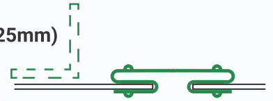
T-7 DOUBLE "S" SLIP (T-7a REINFORCED)
