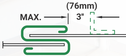
T-6 HEMMED "S" SLIP (T-6a REINFORCED)
